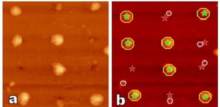
Figure 8: (a) ( 2.5 \mu\text{m} \times 2.5 \mu\text{m} ) images of the island morphology and position on a FIB patterned surface showing domes and pyramids. (b) schematics of islands positions of panel (a) showing pyramids as small circles, domes as large octagons and visible/hidden FIB holes as red/green stars.
