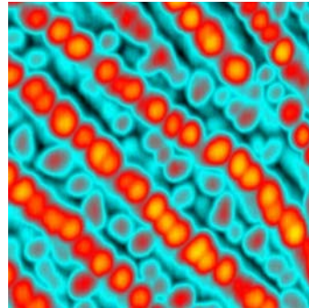
Fig 4 AFM false colour image of nicely ordered ultrasmall Ge islands of lateral size below 50 nm obtained by MBE on a Ge 0.5 Si 0.5 /Si(118) substrate pattern covered by 0.5 ML Sb. Image size 0.5x0.5 \mu\text{m}^2 [Ref. 10]
