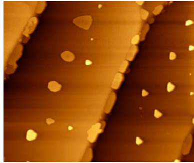
Fig 3 STM image of Ge/Si(111) ordered islands grown by Molecular Beam Epitaxy on self-organized substrate steps at 450 °C. Image size: 2.9x2.9 \mu\text{m}^2 . [Ref. 11]
