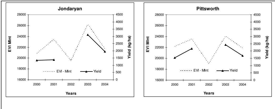
Figure 8 - Estimated yields (kg/ha) from ABS and ABARE and the mean EVI integrated (MInt) during the crop season in the Jondaryan shire for cropping threshold mask, 2000 to 2004
