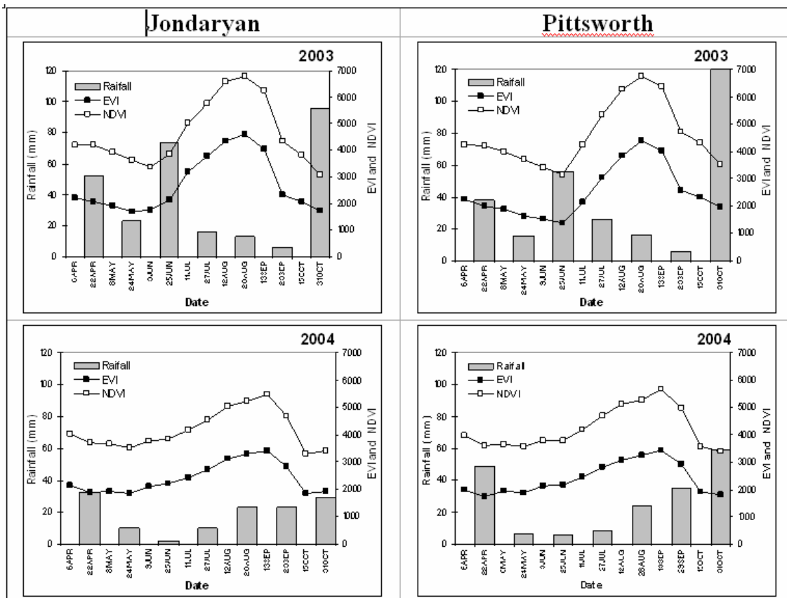
Figure 7 - Monthly rainfall, NDVI and EVI profile ( cropping threshold CMs) from April to November, in Jondaryan and Pittsworth shires, 2003 and 2004.
