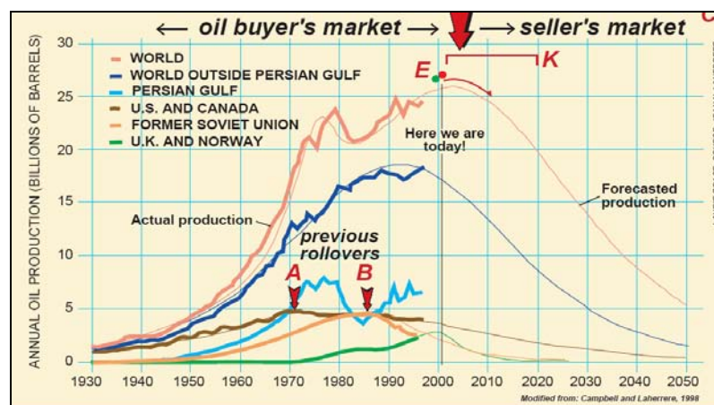
Figure 6 The 'Big Rollover' in the production of conventional oil
