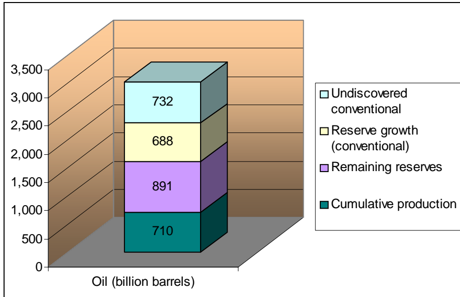
Figure 9 World conventional endowment of oil
